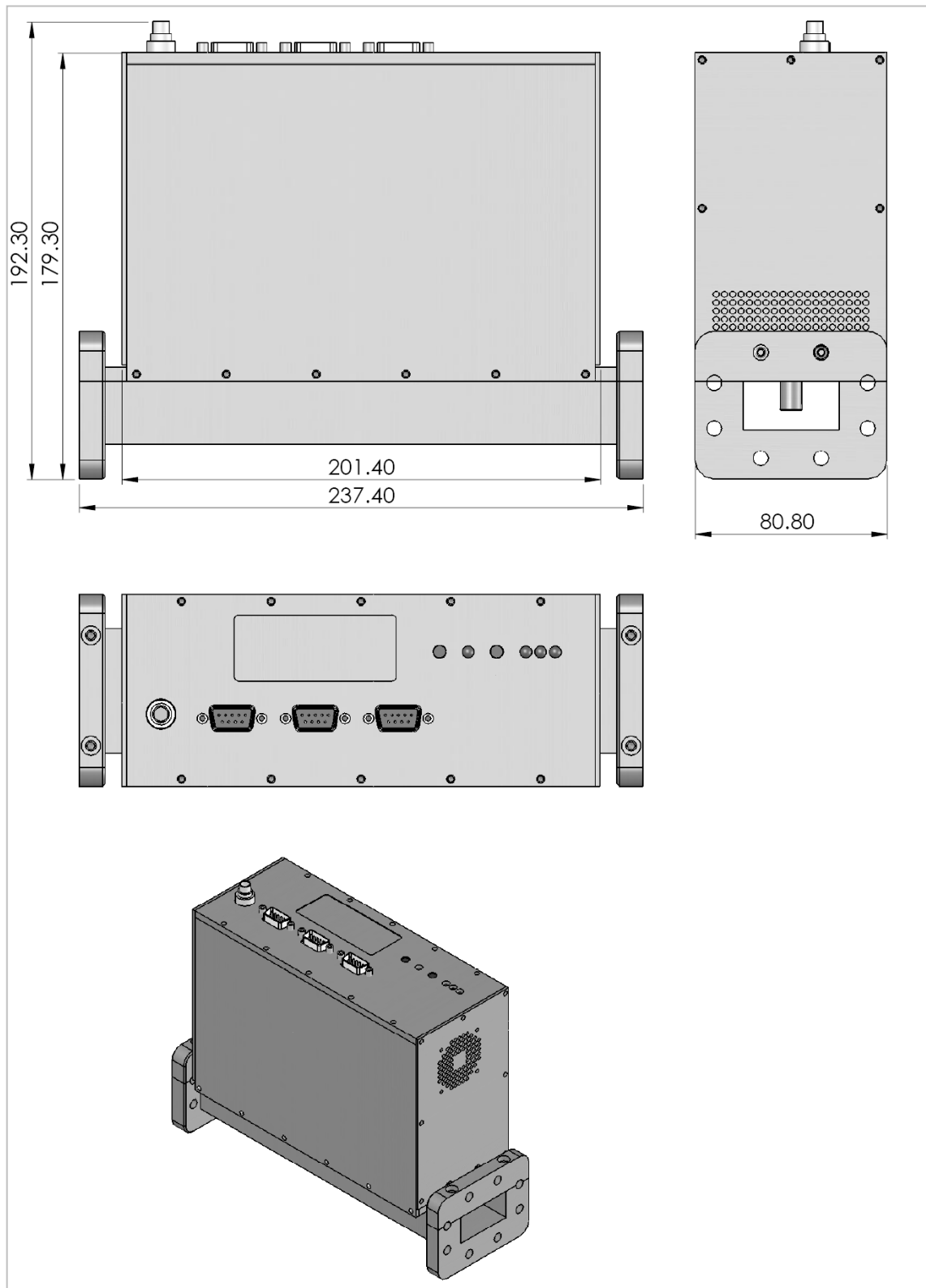
Fig. 4. Basic dimensions of STHT 3.1. All dimensions are in millimeters.
