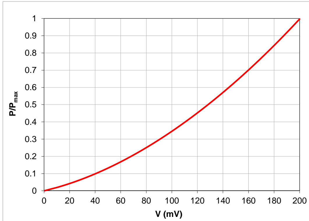
Fig. 3. Typical BD112 correction curve for both directions. P_{\max} is the specified maximum working power.
