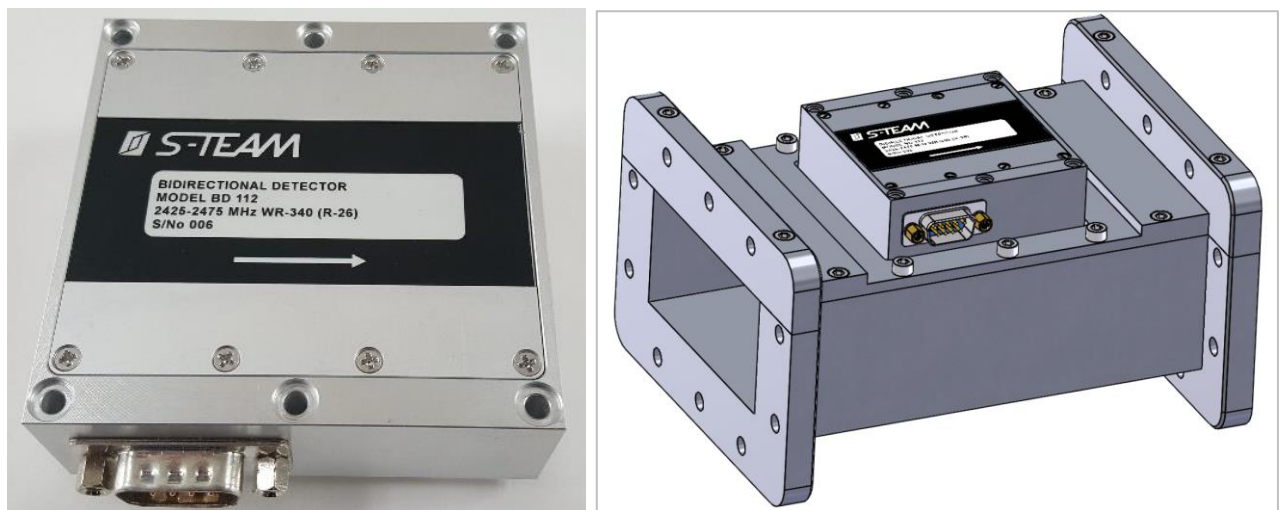
Fig. 1. Left: Bidirectional detector BD112/BD112T. Right: An assembly with a parent waveguide.
