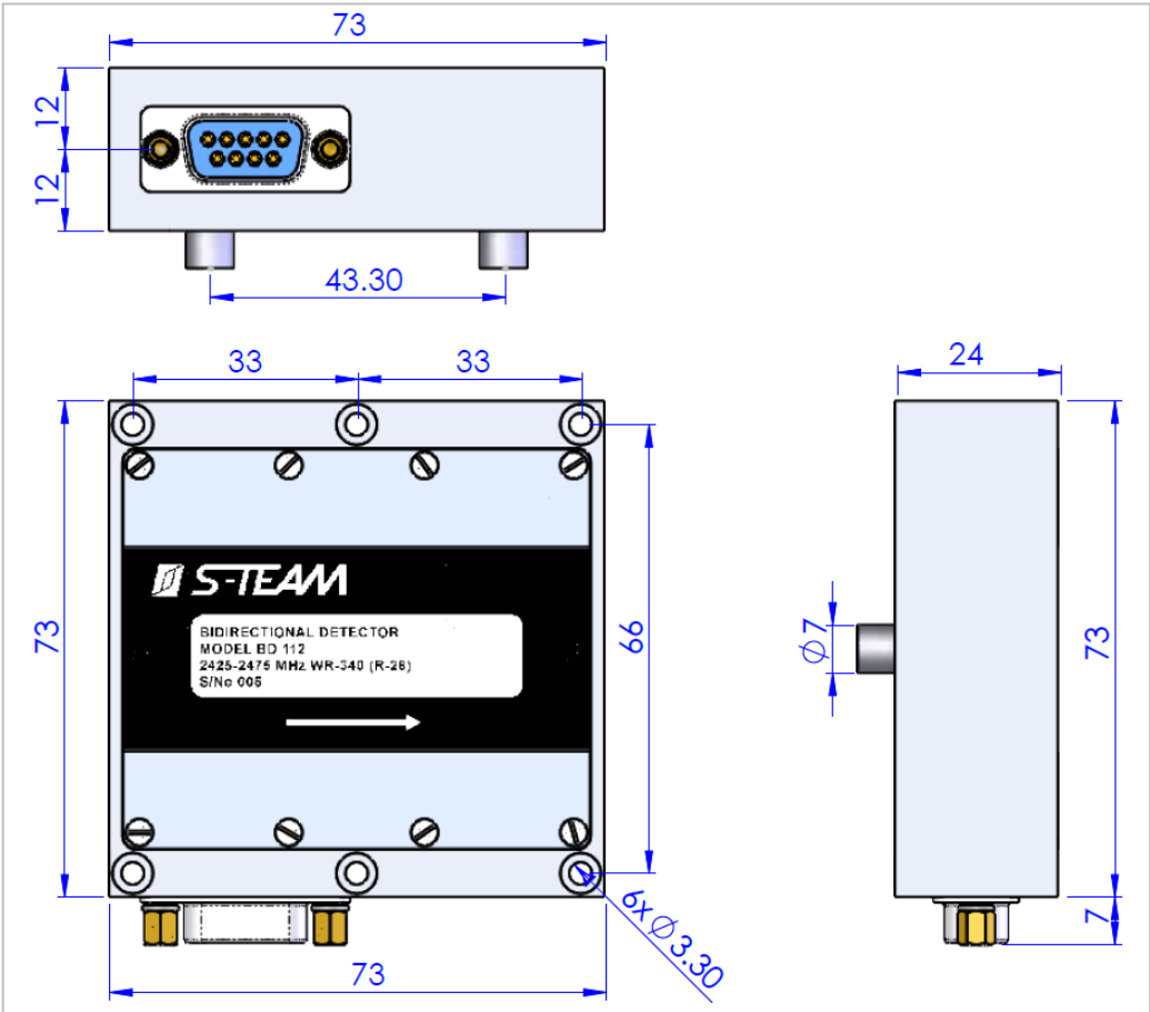
Fig. 5. Basic BD112/BD112T dimensions. All dimensions are in millimeters. The probe protrusion is 5.5 mm.
