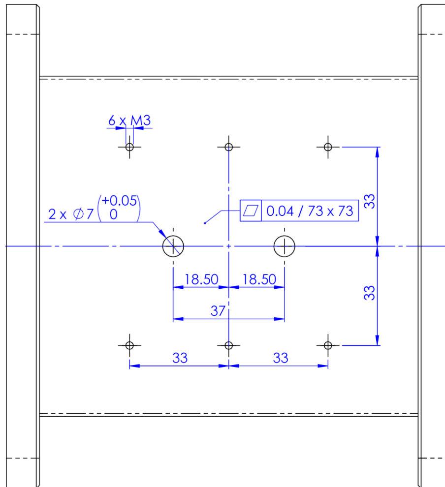
Fig. 6. Waveguide machining template. All dimensions are in millimeters. The waveguide wall thickness must be 2 mm.
