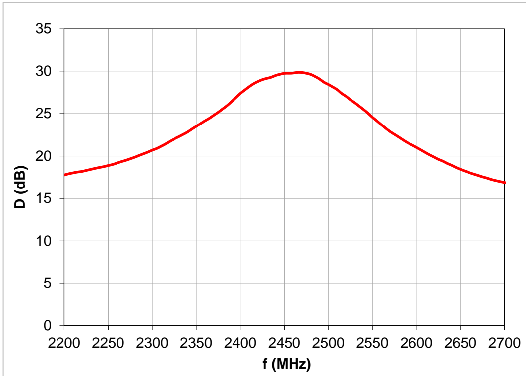
Fig. 4. Typical BD132B directivity (both directions).
