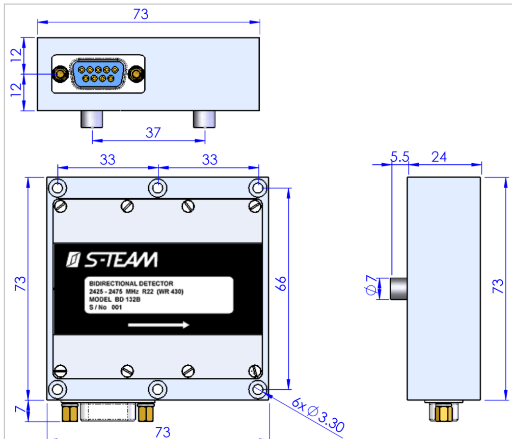
Fig. 5. Basic BD132B dimensions. All dimensions are in millimeters.
