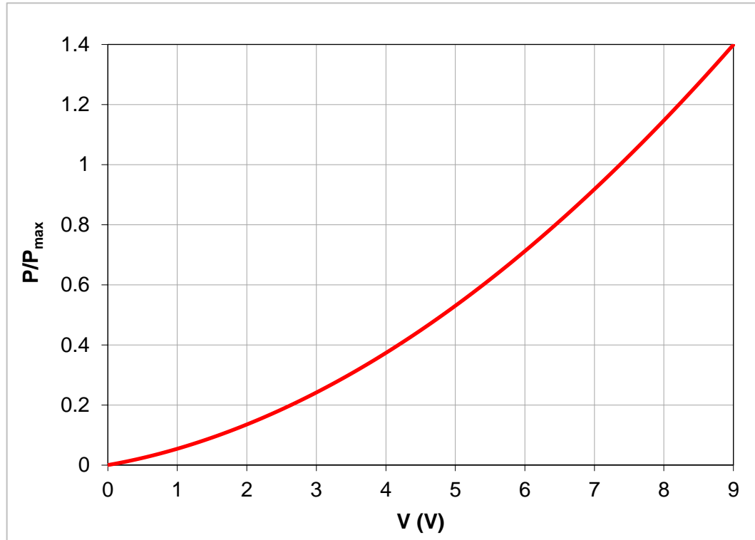
Fig. 3. Typical BD132B correction curve for both directions. P_{\max} is the specified maximum working power.
