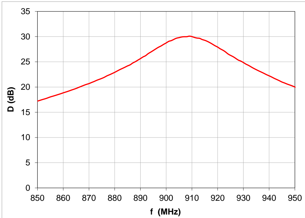
Fig. 5. Typical BD214 directivity (both directions).
