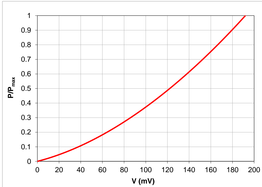
Fig. 4. Typical BD214 correction curve for both directions. P_{\max} is the specified maximum working power.
