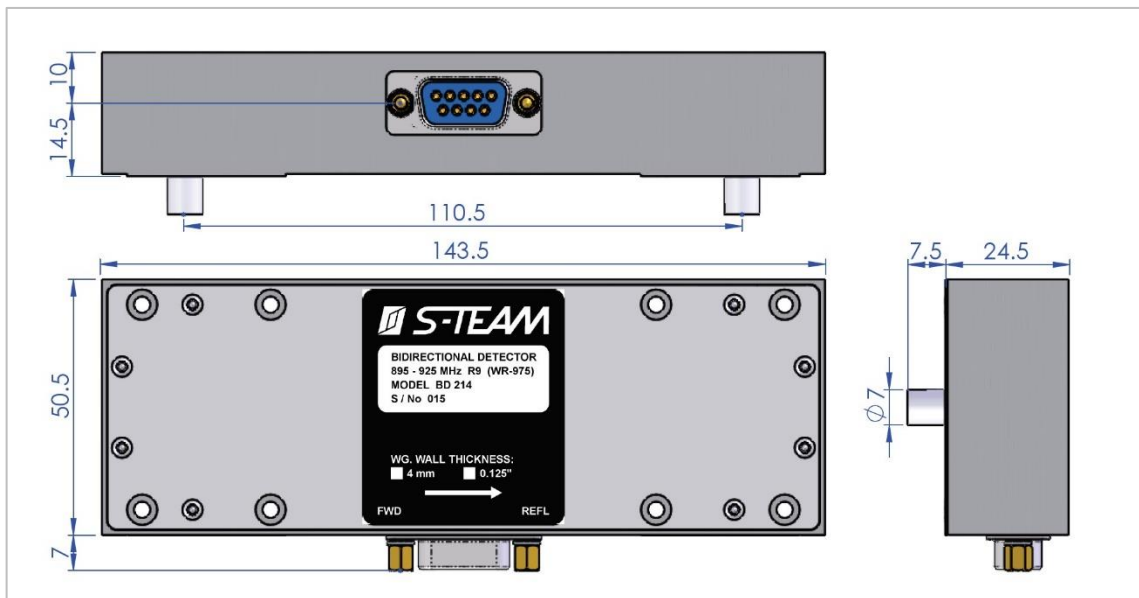
Fig. 6. Basic BD214 dimensions. All dimensions are in millimeters.
