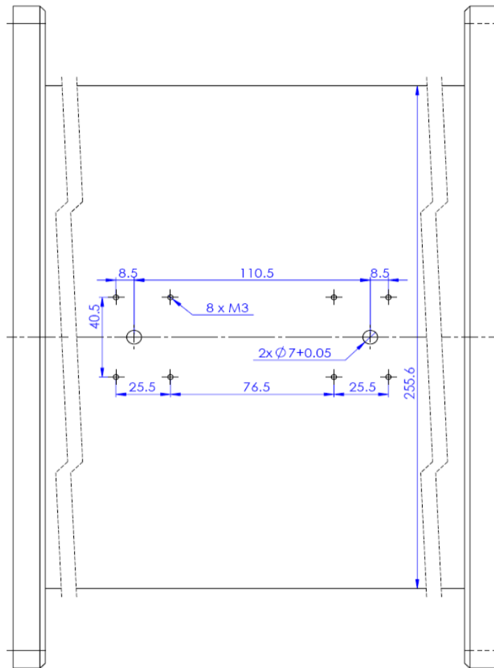
Fig. 5. Waveguide machining template. All dimensions are in millimeters. The pattern is centered about the waveguide axis. Unless the option 0.125" is requested, the waveguide wall thickness must be 4 mm. Suggested screws: M3 x 13 or M3 x 12 (stainless or galvanized steel).
