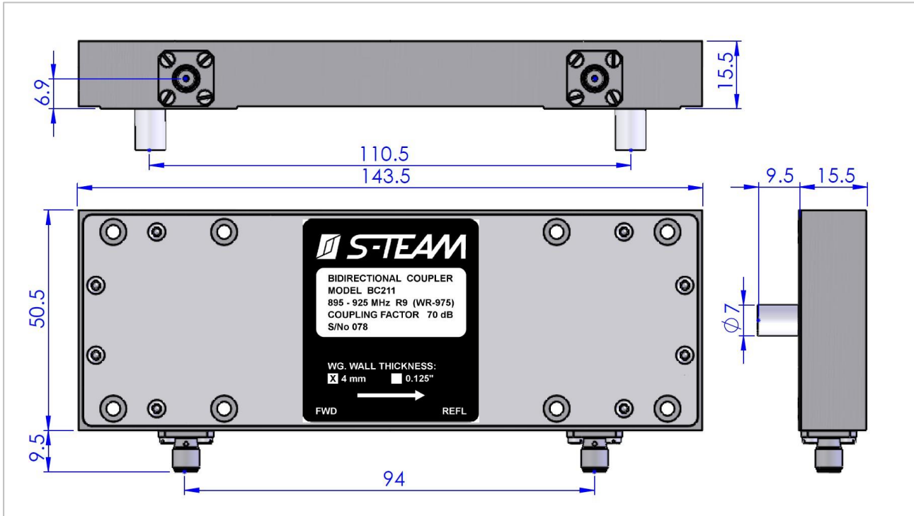
Fig. 4. Basic BC211 dimensions. All dimensions are in millimeters.
