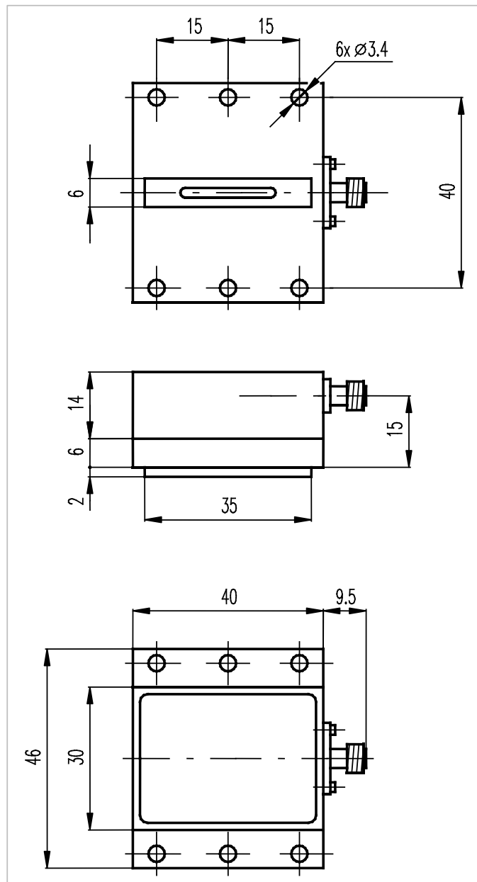
Fig. 3. Basic DD111 dimensions. All dimensions are in millimeters.
