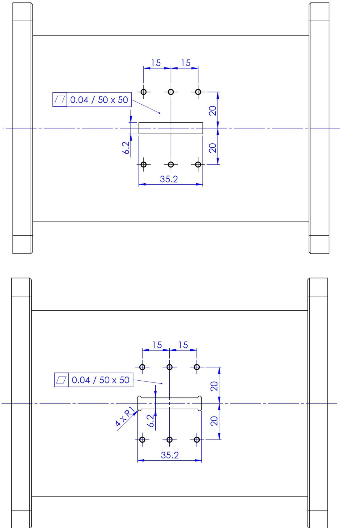
Fig. 4. Waveguide machining template. All dimensions are in millimeters. The bottom alternative is for a better manufacturability. The waveguide wall thickness must be 2 mm . Suggested are M3 x 8 screws (stainless or galvanized steel).
